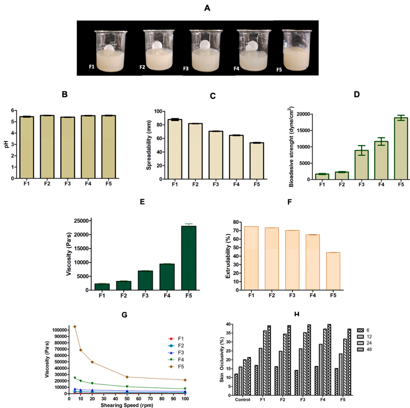
Fig. 7. Formulation of CPL MPs Hydrogel with variation concentration of chitosan (F1: 1 %; F2: 1,25 %; F3: 1,5 %; F4: 1,75 %; F5: 2 %) (A). pH (B), Spreadability (C), Bioadhesive strength (D), Viscosity (E), Extrudability (F), Rheology (G) and Skin occlusivity (H) of CPL MPs hydrogel (means \pm SD, n = 3 ).
