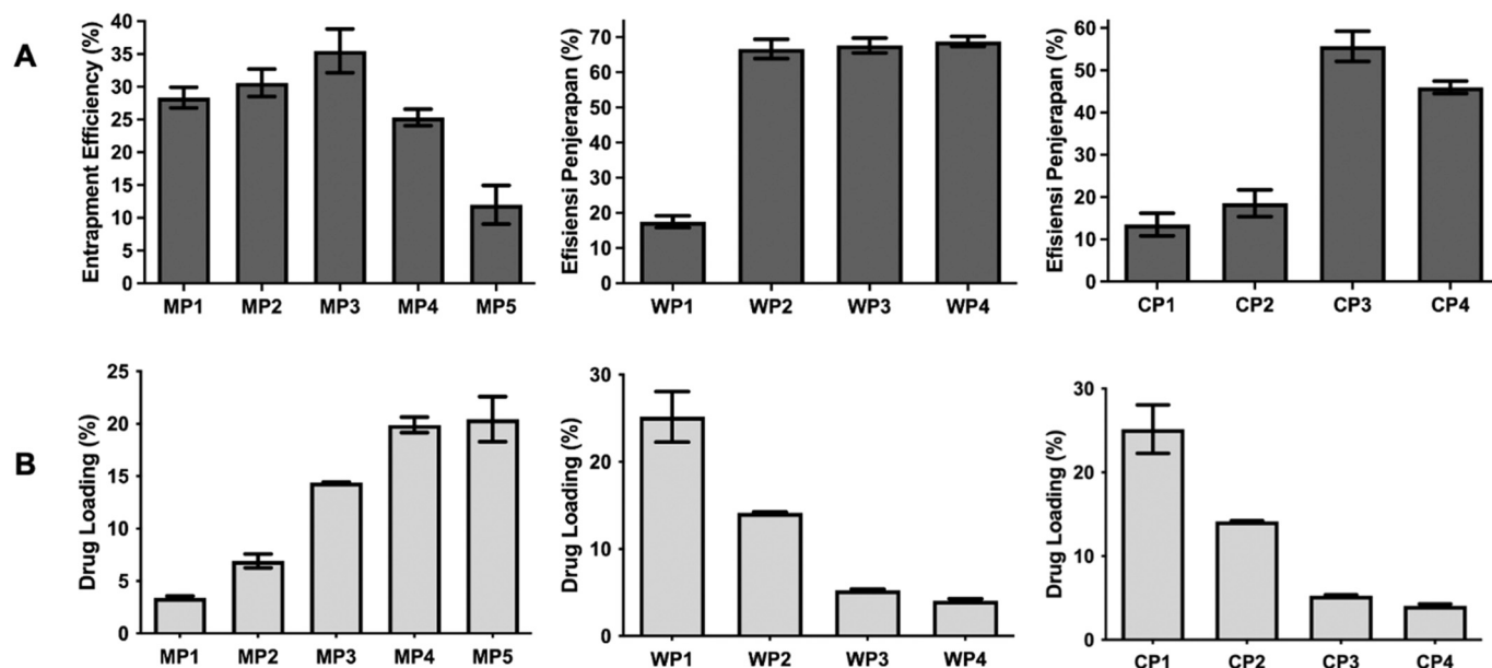
Fig. 3. EE (A) and DL (B) of diagram of CPL MPs with a variation of CPL, WPI and ratio of CPI: WPI concentration (means \pm SD, n = 3 ).
